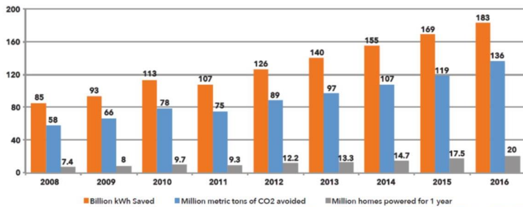
Figure 1. U.S. Energy Efficiency Savings and Carbon Dioxide (CO 2 ) Emissions Avoided (2008-2016)
